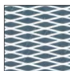
Wire : 4.5mm SWD: 24mm LWD: 60mm
